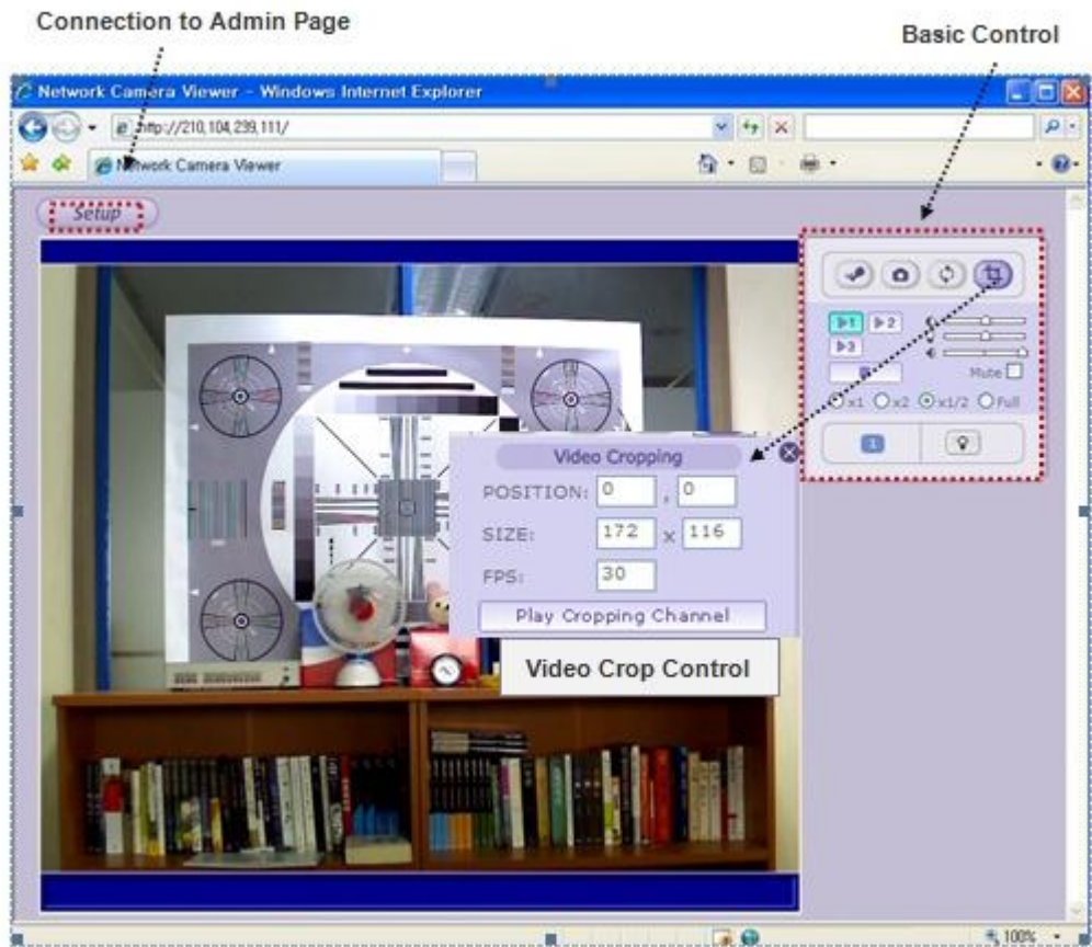
Figure 4-2. Web Viewer
