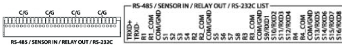
[Figure 2-3 . SVR-1648D1 series Terminal Block and Description]
