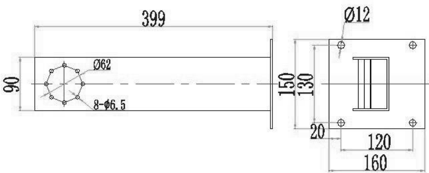
Wall bracket
