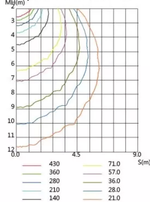
Space Illuminance Curve
